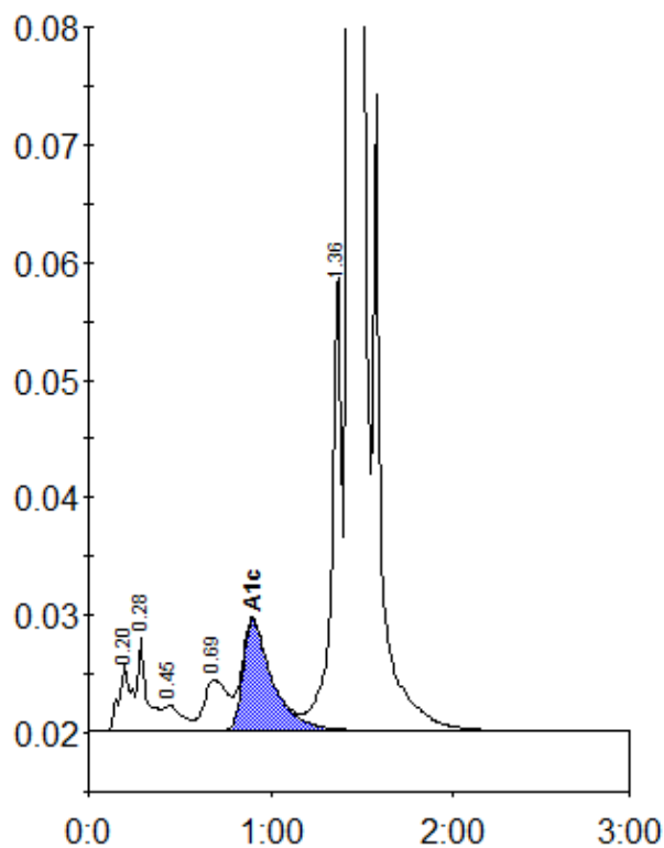
Peak table - ID: 10441129
